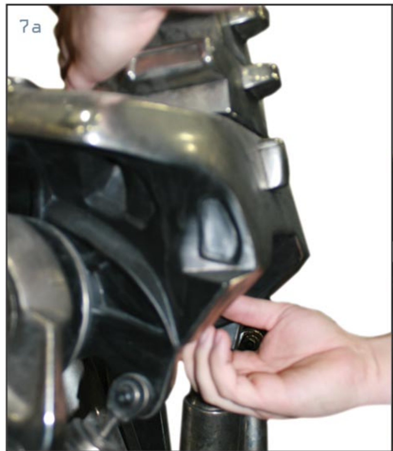
ADD NUT AND HAND-TIGHTEN
