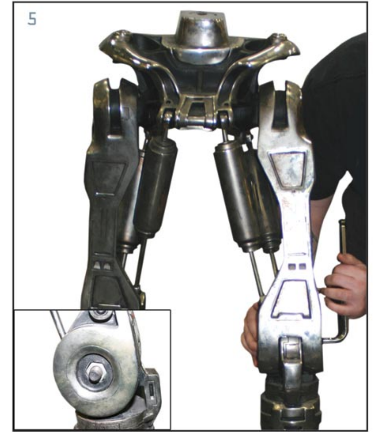
INSERT KNEE BOLT AND TIGHTEN NUT (LEFT & RIGHT)
