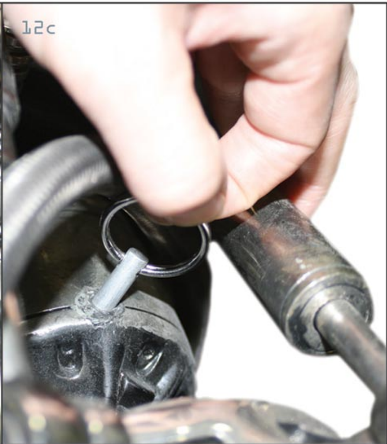
INSERT RETAINING PIN TO LOCK ARM IN POSITION. TO CHANGE ARM POSE, REMOVE THE 'RETAINING PIN,' THEN REMOVE THE ARM. REINSTALL THE ARM AT THE DESIRED POSITION AND INSERT THE RETAINING PIN
