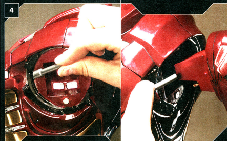
4 PLACE LEFT ARM PISTON INTO HOLE, HOLD PISTON AND CONNECT LEFT ARM TO SHOULDER. REPEAT STEPS FOR RIGHT ARM.
